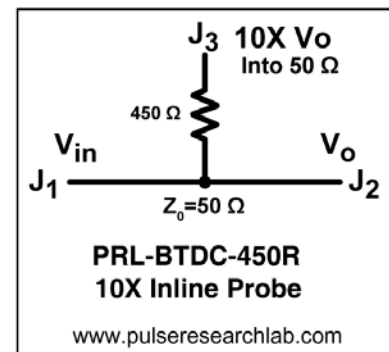
Figure 3: PRL-BTDC-450R Block Diagram
